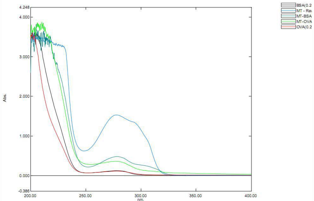
Figure 2. UV-spectrum
